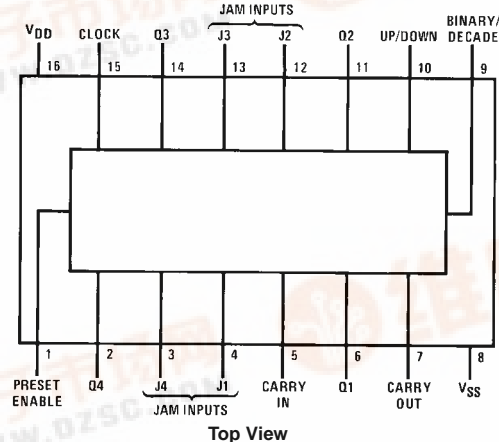
Pin Assignments for DIP, SOIC and SOP
