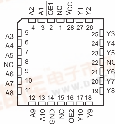
SN54BCT29827B . . . FK PACKAGE (TOP VIEW)
