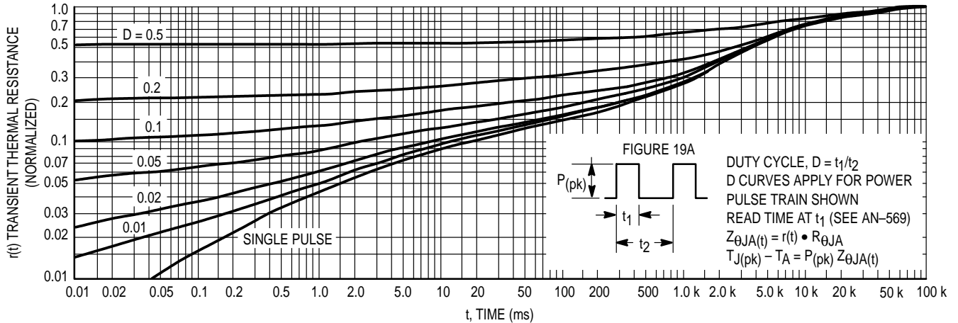
Figure 19. Thermal Response
