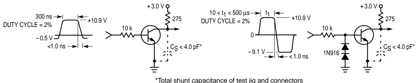
Figure 1. Turn–On Time
