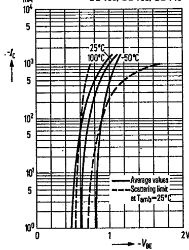
Collector current I_C = f(V_{CE}) V_{CE} = 2V ; T_{amb} = parameter (common emitter configuration) BD 136, BD 138, BD 140
