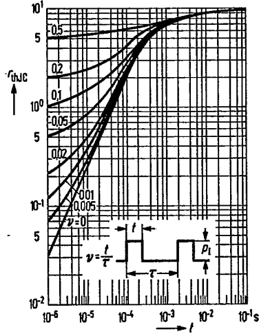
Permissible pulse load r_{thJC} = f(t) ; v = parameter BD 136, BD 138, BD 140
