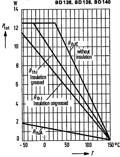
Total perm. power dissipation versus temperature P_{tot} = f(T) ; R_{th} = parameter BD 136, BD 138, BD 140
