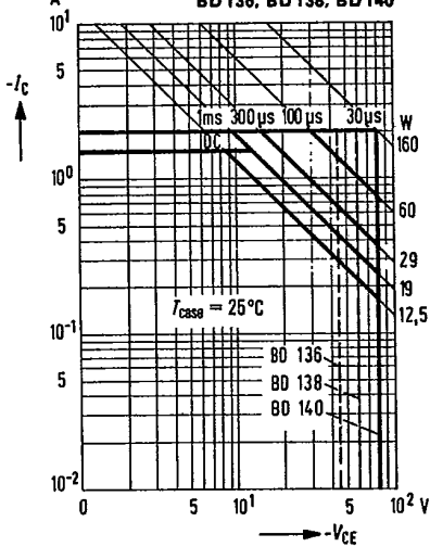
Permissible operating range I_C = f(V_{CE}) ; ( T_{case} = 60^\circ C ); v = 0 BD 136, BD 138, BD 140
