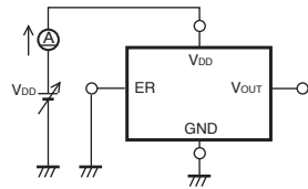
I/O characteristic
