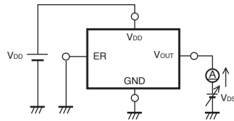
Detection voltage
