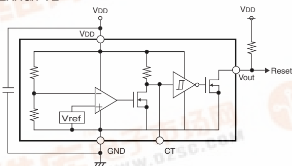
BD52XXG/FVE
