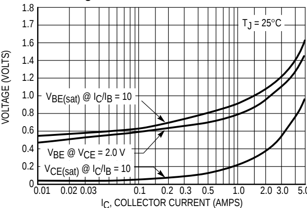
Figure 4. "On" Voltage
