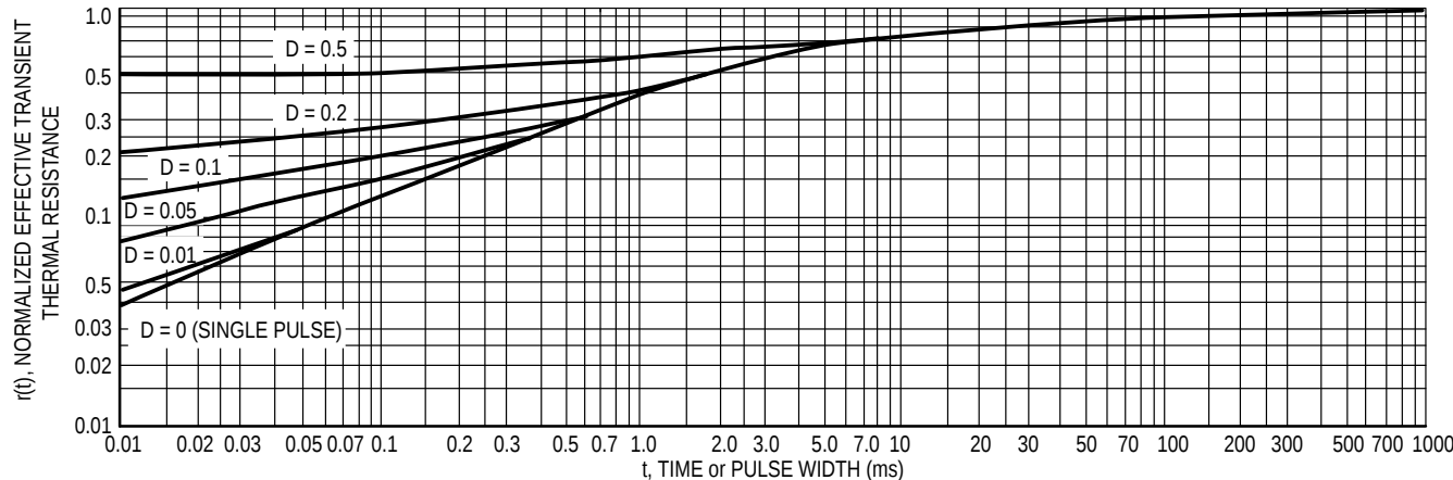
Figure 5. Thermal Response
