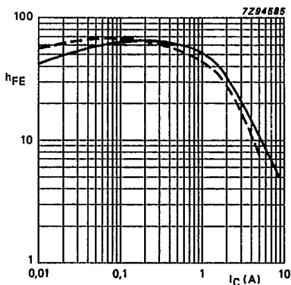
Fig. 9 D.C. current gain; V_{CE} = 2V ; typical values; — T_j = 25^{\circ}C ; --- T_j = 125^{\circ}C .
