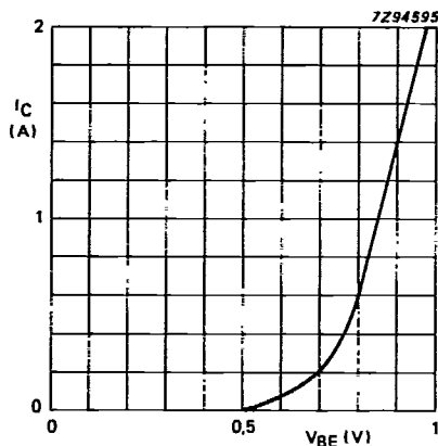
Fig. 10 V_{CE} = 2V ; typical values.
