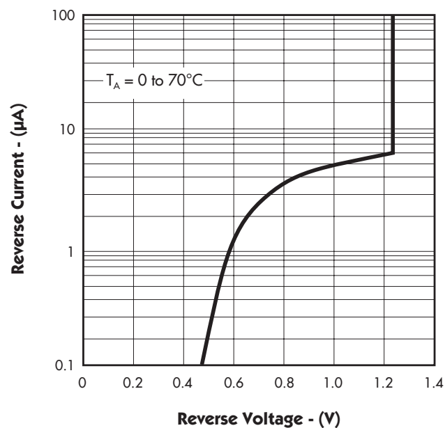
FIGURE 2. — REVERSE CHARACTERISTICS
