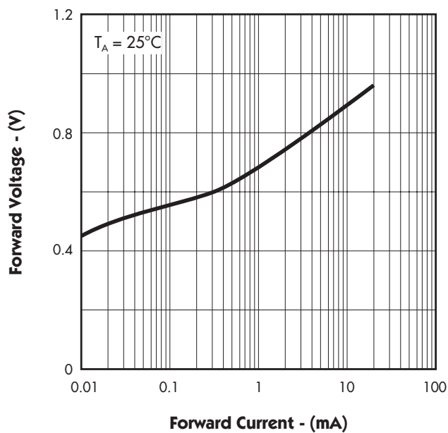
FIGURE 3. — FORWARD CHARACTERISTICS
