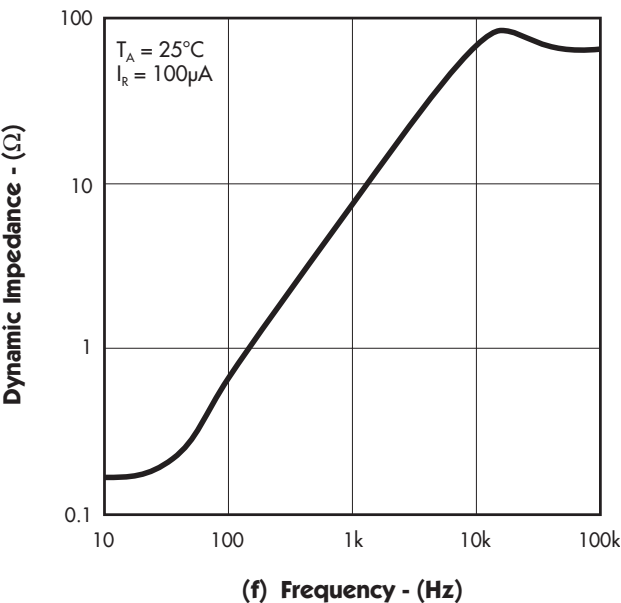
FIGURE 12. — REVERSE DYNAMIC IMPEDANCE
