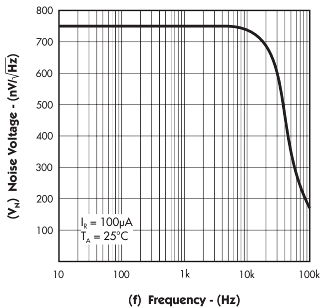
FIGURE 7. — NOISE VOLTAGE
