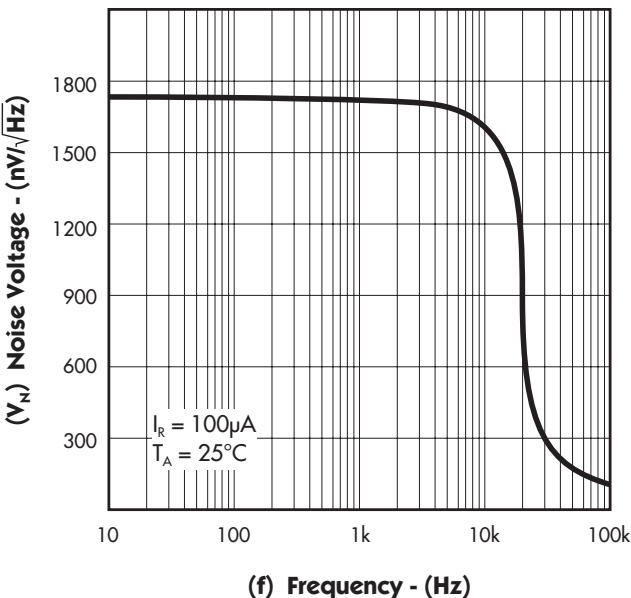
FIGURE 13. — NOISE VOLTAGE
