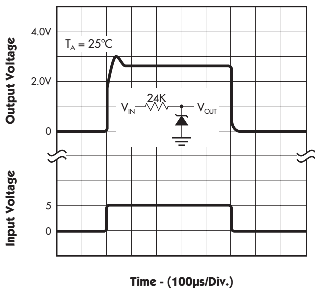
FIGURE 8. — RESPONSE TIME
