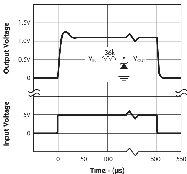
FIGURE 1. — RESPONSE TIME
