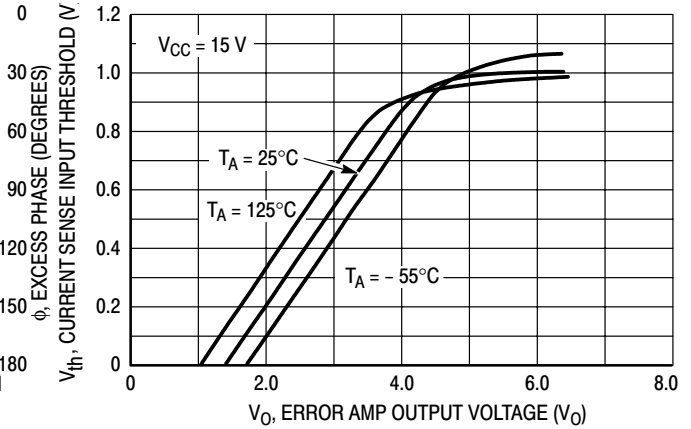
Figure 7. Current Sense Input Threshold versus Error Amp Output Voltage
