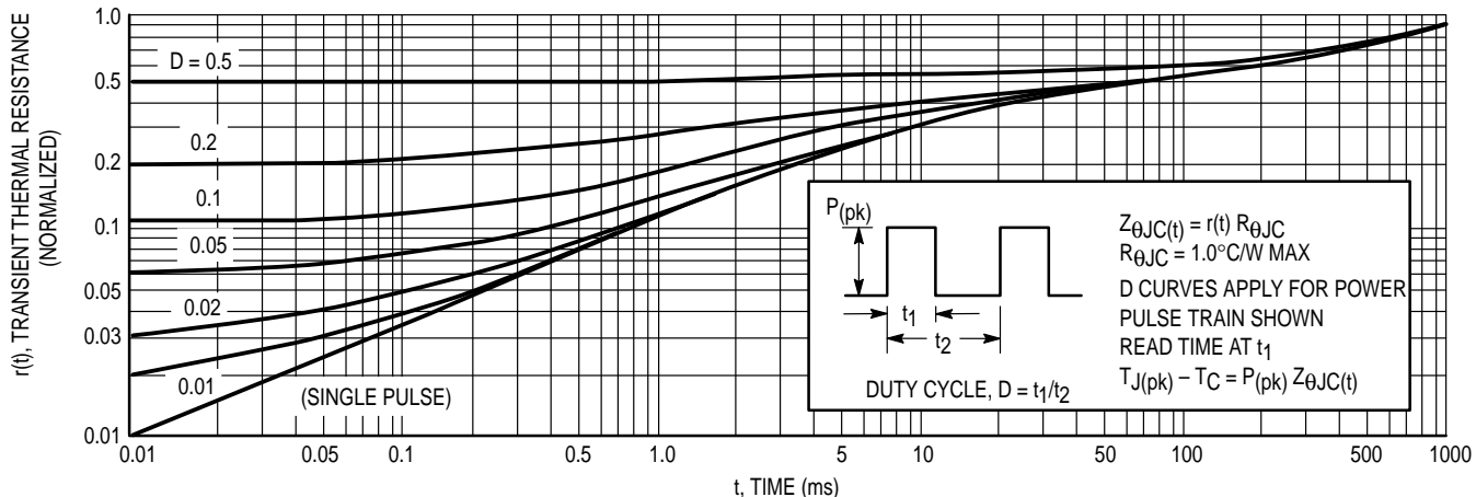
Figure 7. Thermal Response
