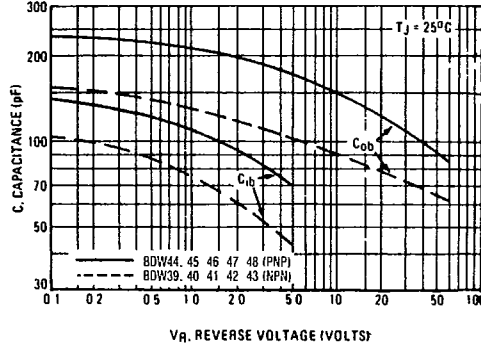
FIGURE 8 - CAPACITANCE
