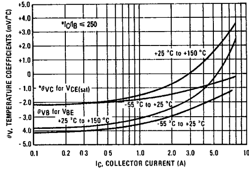
FIGURE 12 -- TEMPERATURE COEFFICIENTS
