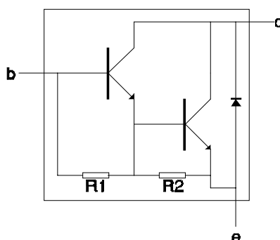
Circuit diagram.
