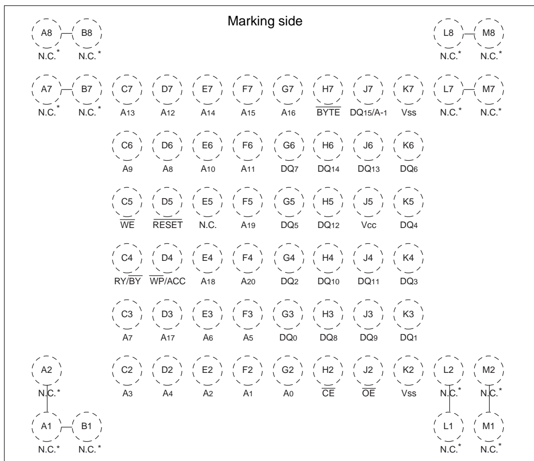
FBGA (TOP VIEW)
