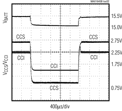
LOAD-TRANSIENT RESPONSE (STEP-IN LOAD CURRENT)
