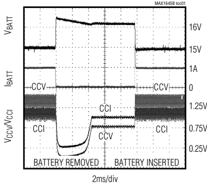
BATTERY REMOVAL AND REINSERTION TRANSIENT RESPONSE
