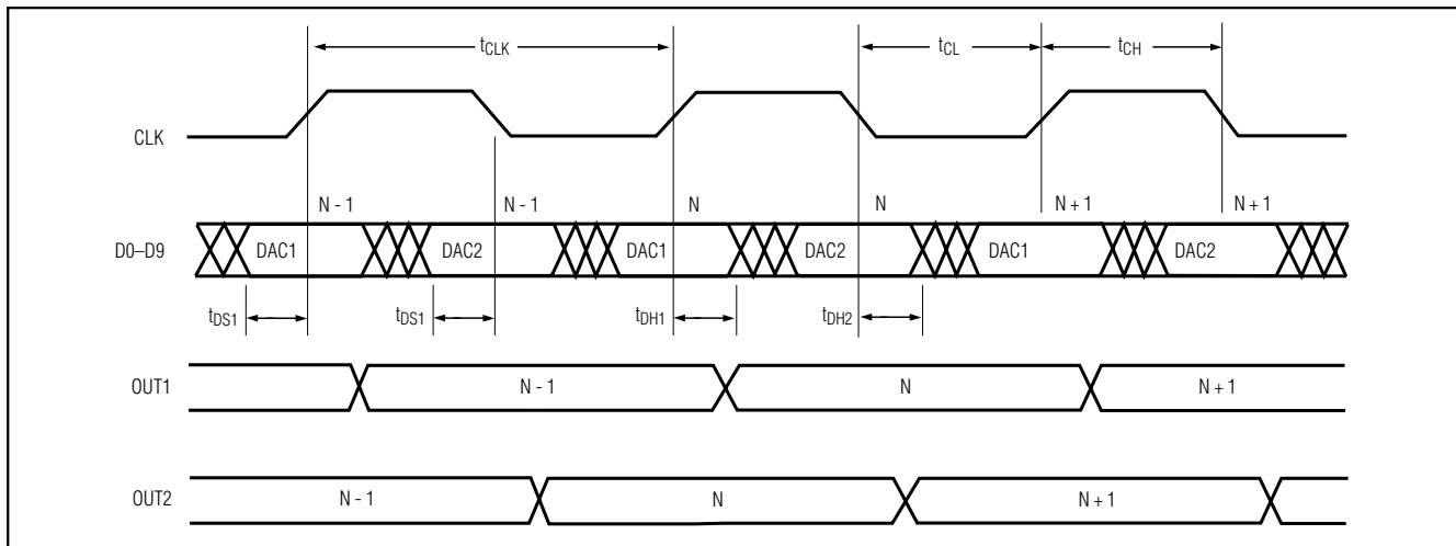
Figure 4. Timing Diagram
