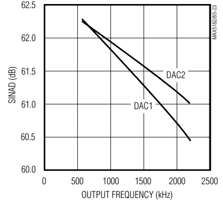
SIGNAL-TO-NOISE PLUS DISTORTION vs. OUTPUT FREQUENCY
