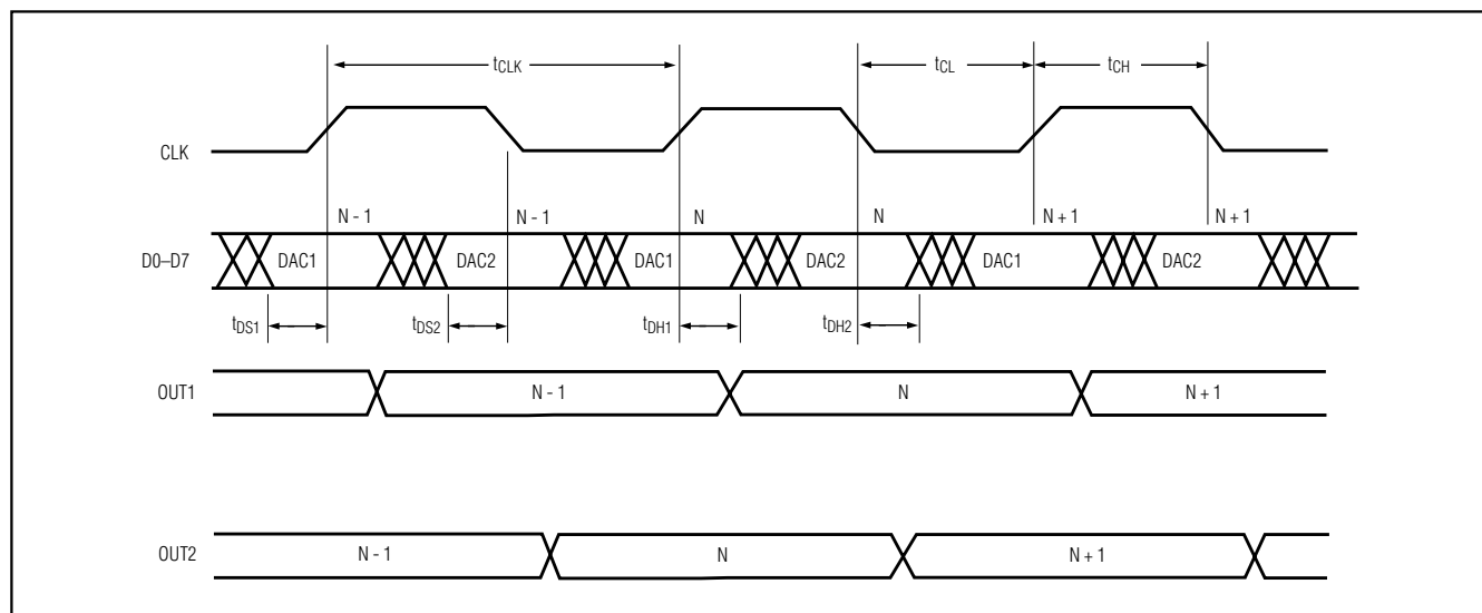
Figure 4. Timing Diagram
