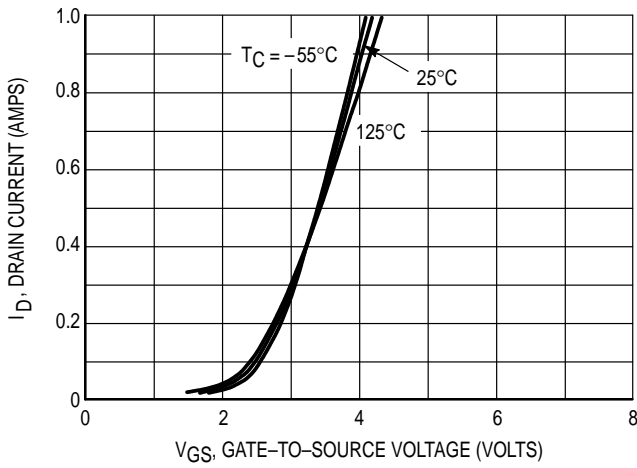
Figure 1. Transfer Characteristics
