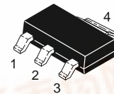
CASE 318E-04, STYLE 1 SOT-223 (TO-261AA)
