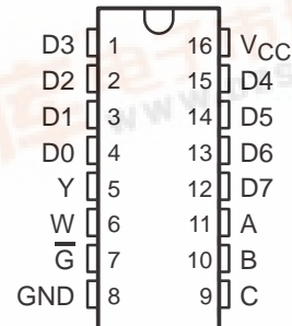
SN54F151B ... J PACKAGE SN74F151B ... D OR N PACKAGE (TOP VIEW)
