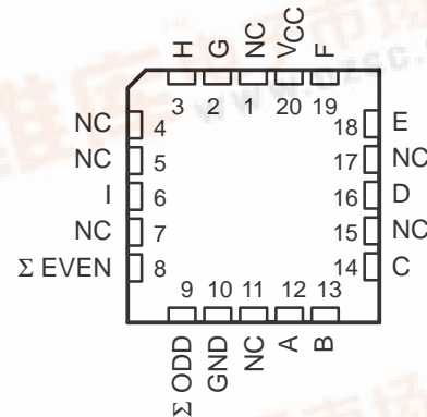
SN54F280B ... FK PACKAGE (TOP VIEW)
