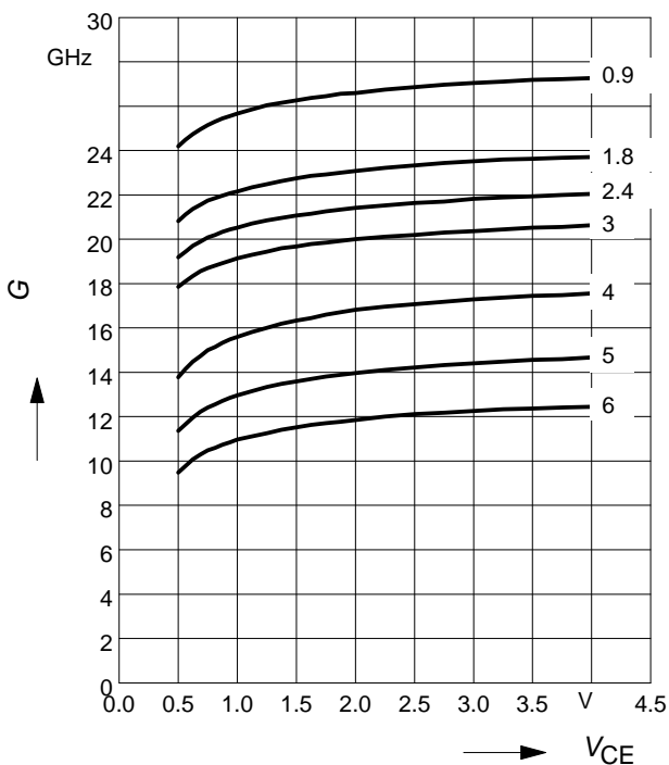
Power gain G_{ma}, G_{ms} = f(V_{CE}) I_C = 5\text{ mA} f = \text{parameter in GHz}
