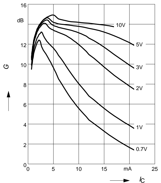
Power Gain G_{ma}, G_{ms} = f(I_C) f = 1.8\text{GHz} V_{CE} = \text{Parameter}
