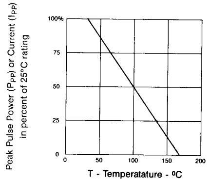
FIGURE 3 DERATING CURVE
