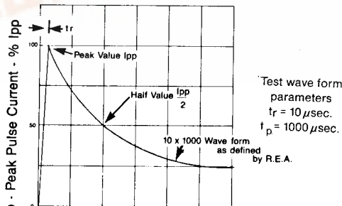
FIGURE 2 PULSE WAVEFORM
