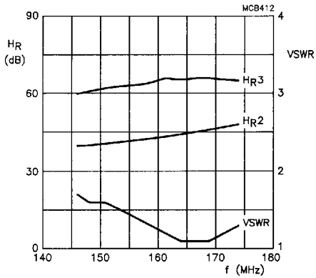
Fig.9 Second and third harmonic rejection as a function of frequency; P_L = 28\text{ W} ; V_{S1} = V_{S2} = 12.5\text{ V} ; typical values.
