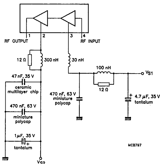
Fig.4 Decoupling arrangement.
