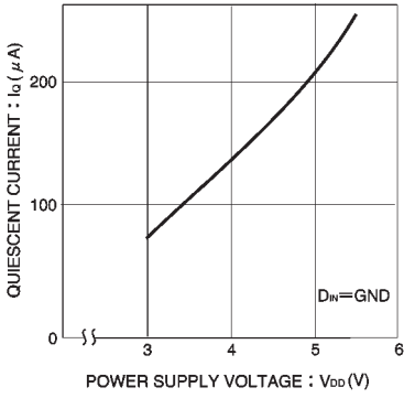
Fig. 4 Power supply voltage vs. quiescent curve
