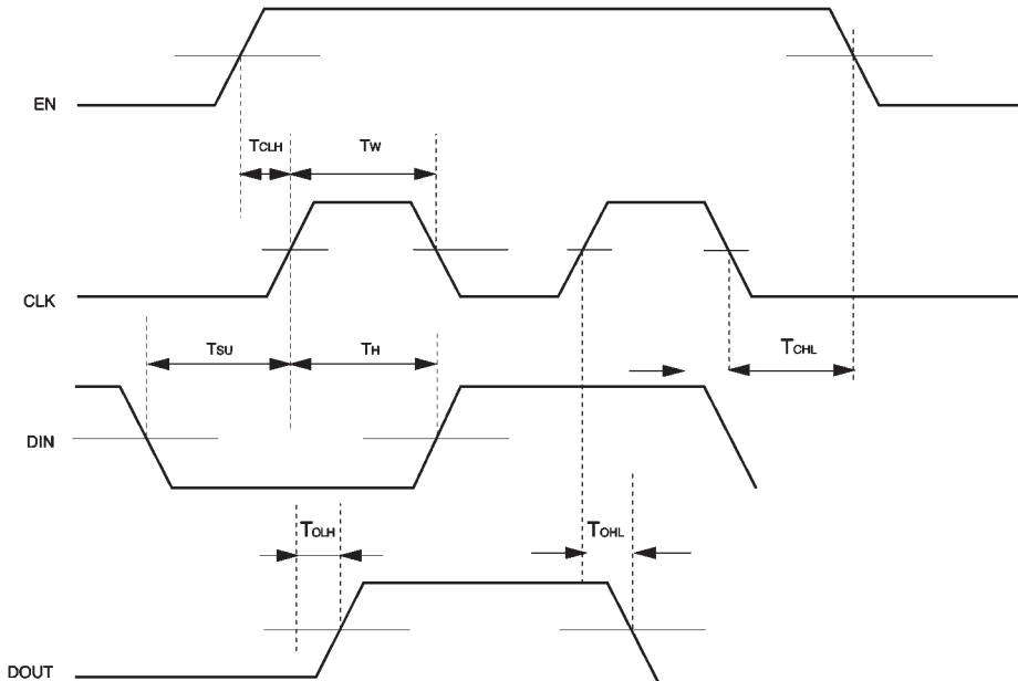
Fig. 2 Timing chart 1
