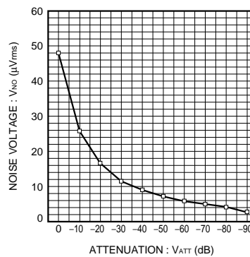
Fig.8 Noise level
