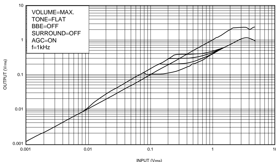
Fig.2 AGC characteristics
