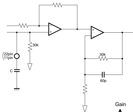
Equivalent Circuit
