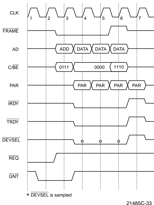
Figure 30. FIFO Burst Write At End Of Unaligned Buffer
