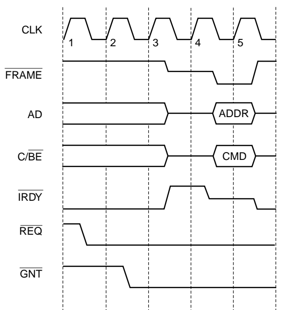
Figure 11. Bus Acquisition
