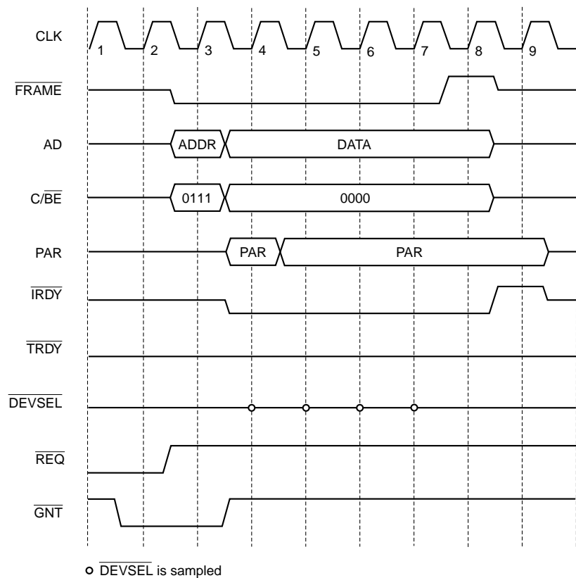
Figure 21. Master Abort
