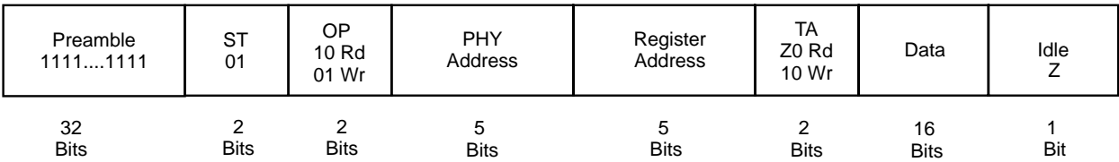
Figure 36. Frame Format at the MII Interface Connection
