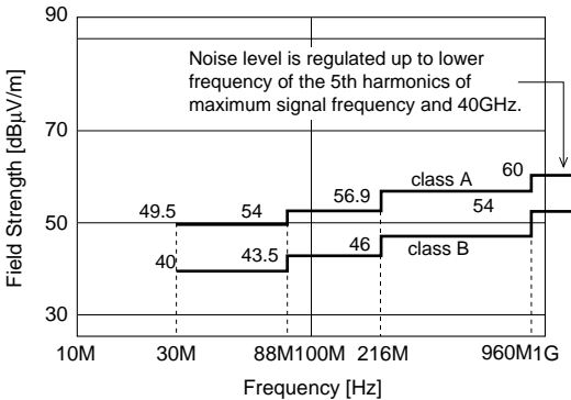
[Radiated Interference]
