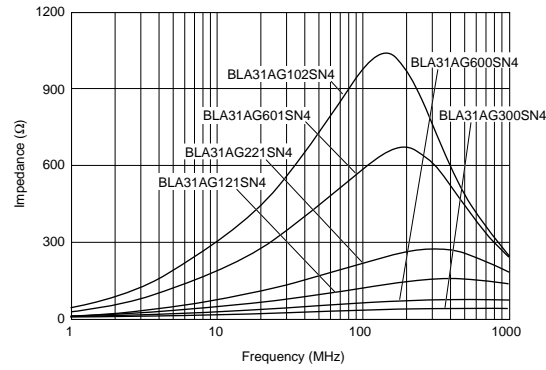
BLA31A Series
