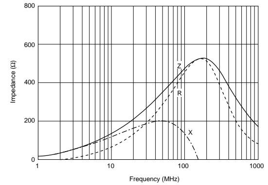
BLM21AG471SN1
