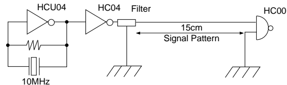
[Testing Circuit]
