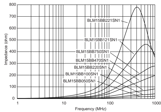
BLM15BB Series
