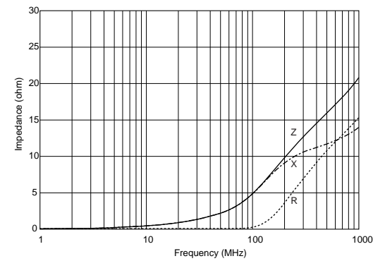
BLM15BB050SN1
