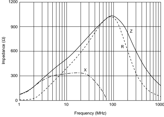
BLM21RK102SN1
