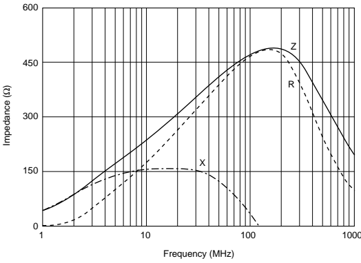
BLM21RK471SN1
