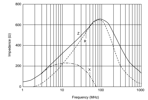
BLM21AJ601SN1
