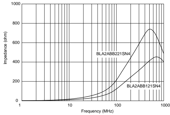
BLA2ABB Series
