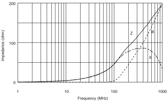
BLA2ABB470SN4
