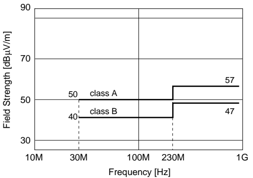
[Radiated Interference]
