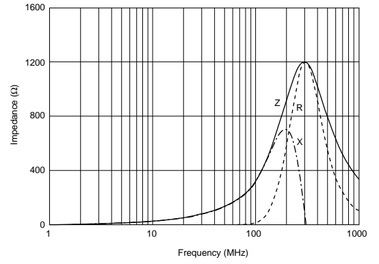
BLM18BB331SN1
