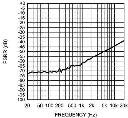
PSRR vs Frequency V_I = 6.1V , Z_L = 2\mu F + 30\Omega , V_{ripple} = 200mV_{pp} , A_{V-BTL} = 26dB
