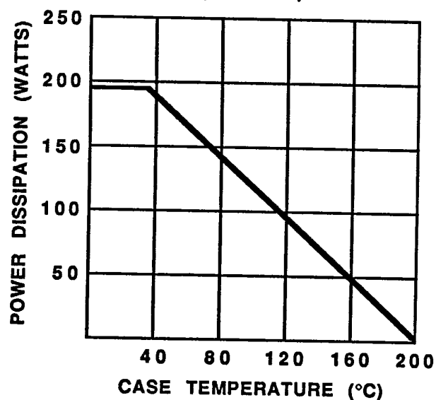
POWER DERATING CURVE (TYPICAL)
