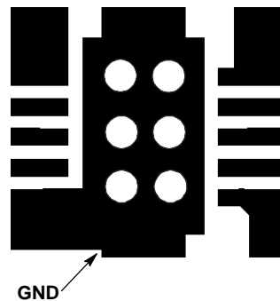
Figure 18. Recommended Footprint
