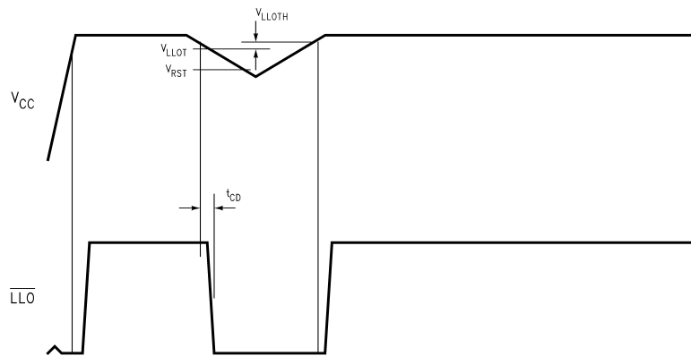
FIGURE 2. \overline{LLO} Output
