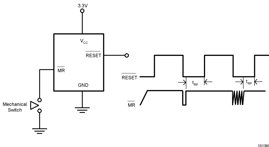
FIGURE 11. Switch Debouncer
