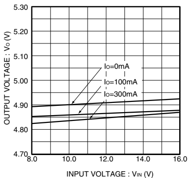
Fig.5 Line regulation
