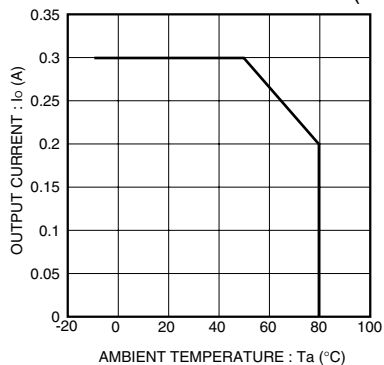
Fig.2 Derating curve
