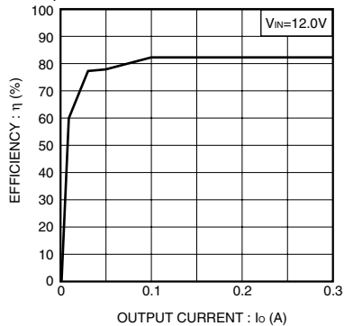
Fig.3 Conversion efficiency
