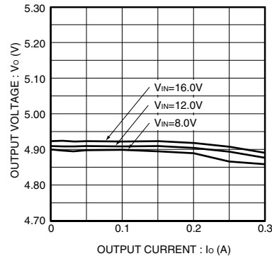
Fig.4 Output characteristic
