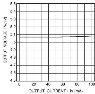
Fig.9 Output characteristic
