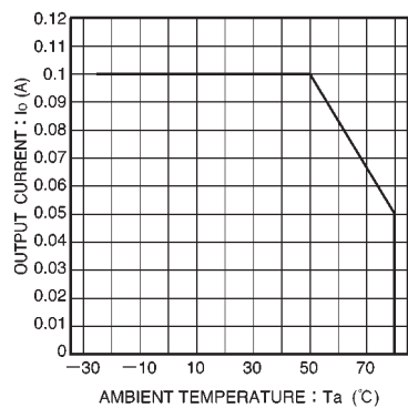
Fig.7 Derating curve
