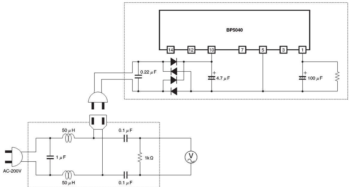
Fig.6 Test circuit
