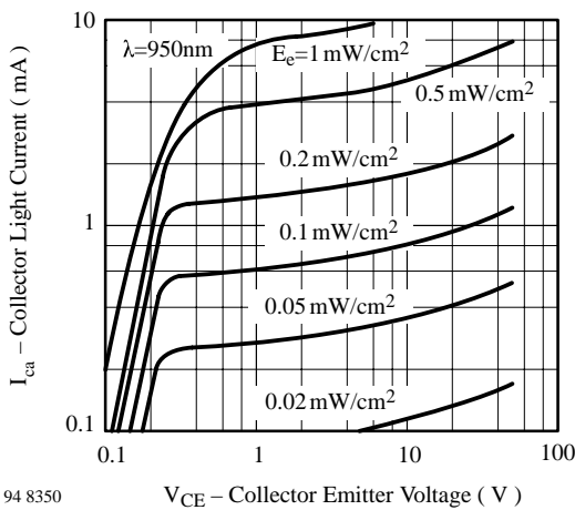
94 8350 V_{CE} – Collector Emitter Voltage ( V ) Figure 5. Collector Light Current vs. Collector Emitter Voltage
