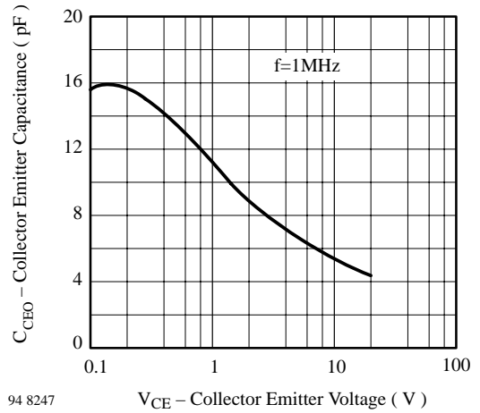
94 8247 V_{CE} – Collector Emitter Voltage ( V ) Figure 6. Collector Emitter Capacitance vs. Collector Emitter Voltage
