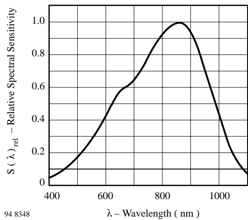
94 8348 \lambda – Wavelength ( nm ) Figure 8. Relative Spectral Sensitivity vs. Wavelength
