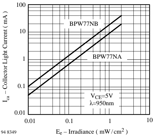
94 8349 E_e – Irradiance ( mW/cm 2 ) Figure 4. Collector Light Current vs. Irradiance
