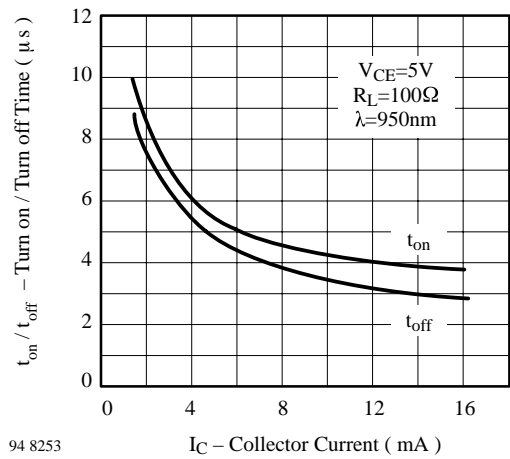
94 8253 I_C – Collector Current ( mA ) Figure 7. Turn On/Turn Off Time vs. Collector Current
