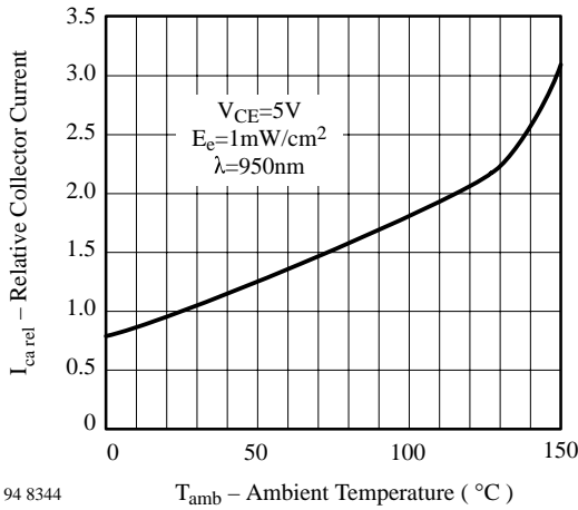
94 8344 T_{amb} – Ambient Temperature ( °C ) Figure 3. Relative Collector Current vs. Ambient Temperature
