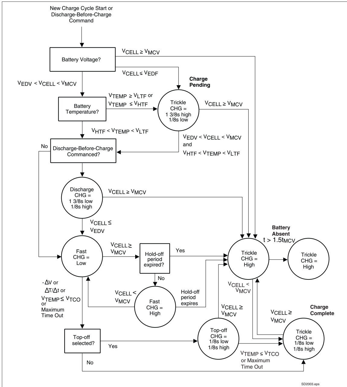
Figure 3. State Diagram
