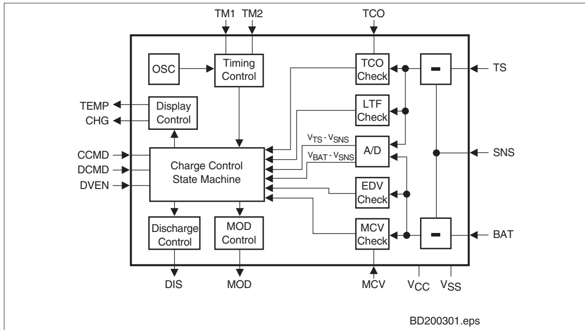
Figure 4. Block Diagram
