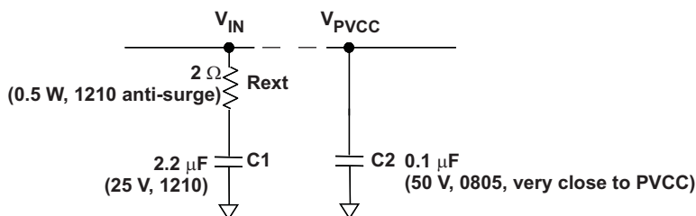
Figure 38. Recommended Input Filter Design
