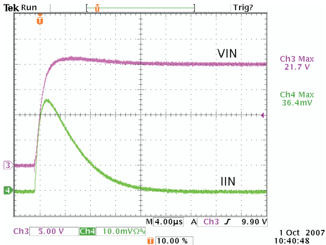
Figure 39. Adapter DC Side Hot Plug-in Test Waveforms
