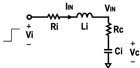
Figure 36. Simplified Equivalent Circuit During Adapter Insertion
