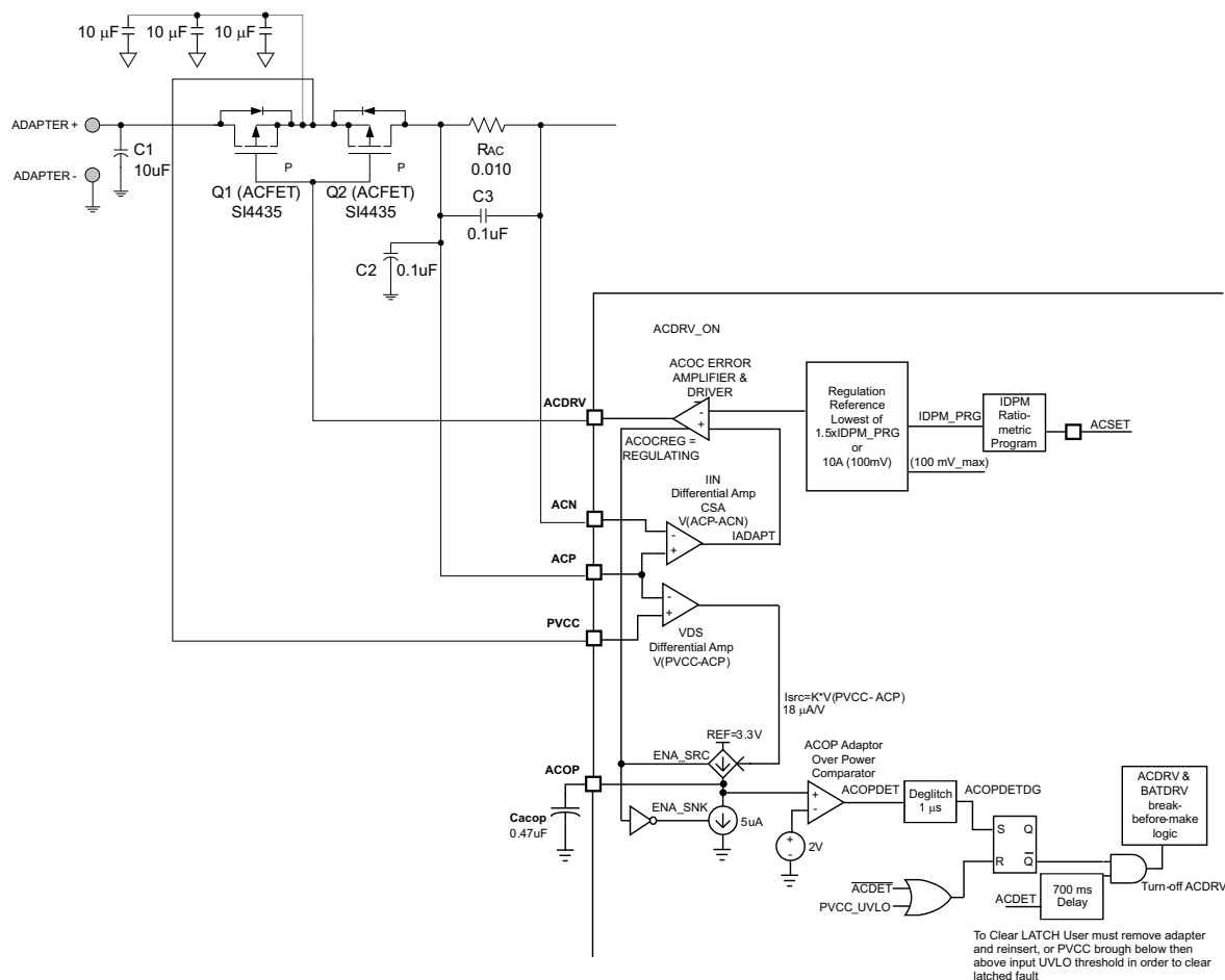
Figure 35. ACOC / ACOP Circuit Functional Block Diagram
