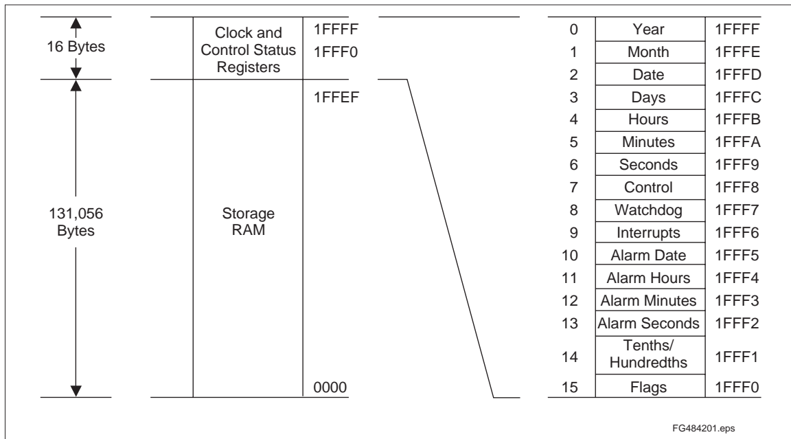
Figure 2. Address Map
