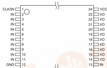
TSSOP Top View
