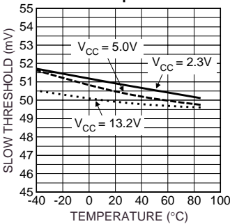
Circuit Breaker Slow ( V_{TRIP} ) vs. Temperature
