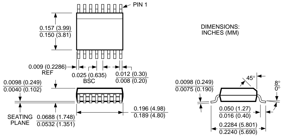
QSOP-16
