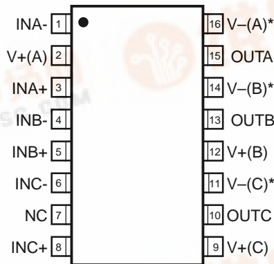
QSOP-16
