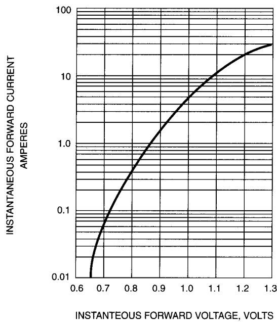
FIG. 3-TYPICAL FORWARD CHARACTERISTICS
