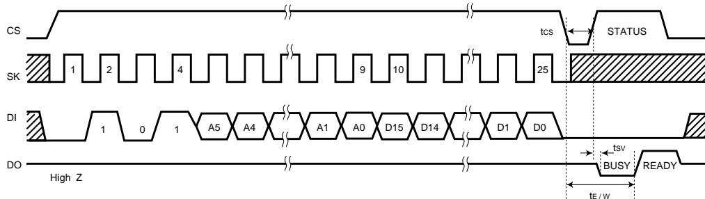
Fig.12 Write cycle timing (WRITE)
