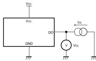
Fig.3 "LOW" output voltage circuit
