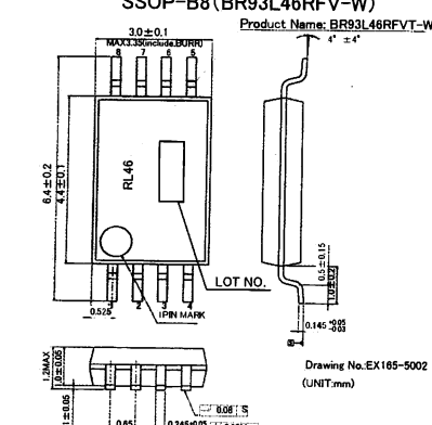
Fig4-(j) PHYSICAL DIMENSION TSSOP-B8 (BR93L46RFVT-W)
