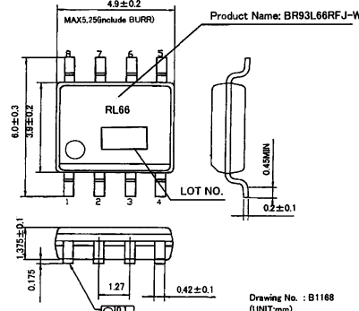
Fig4-(e) PHYSICAL DIMENSION SOP-J8 (BR93L66RFJ-W)
