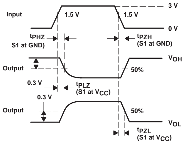
VOLTAGE WAVEFORMS
