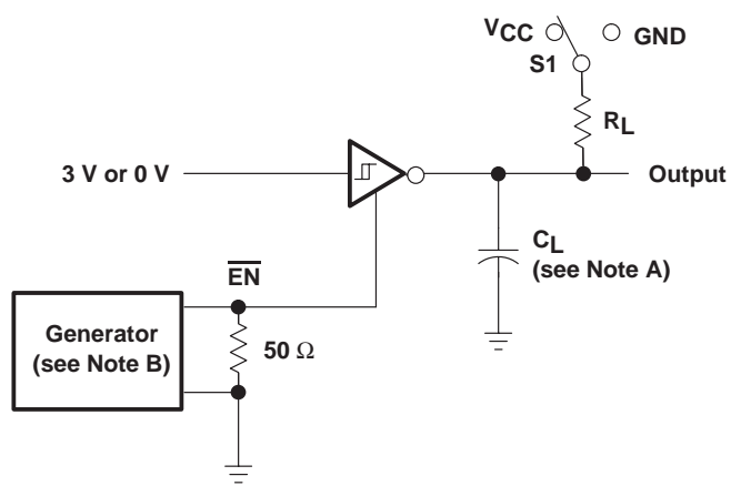
TEST CIRCUIT
