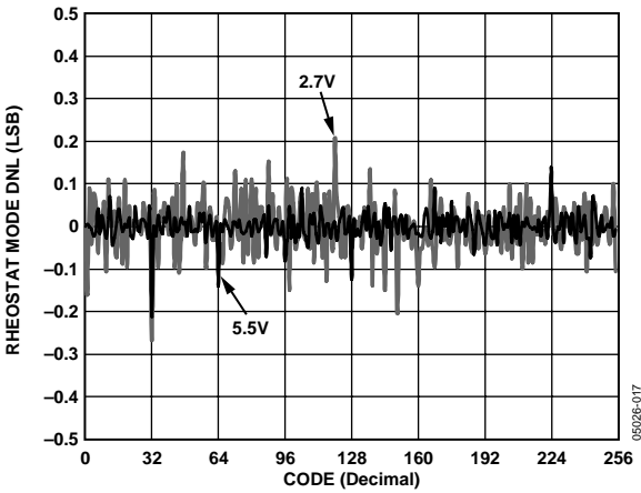
Figure 7. R-DNL vs. Code vs. Supply Voltage
