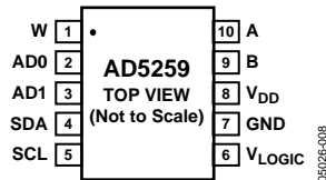
Figure 5. Pin Configuration
