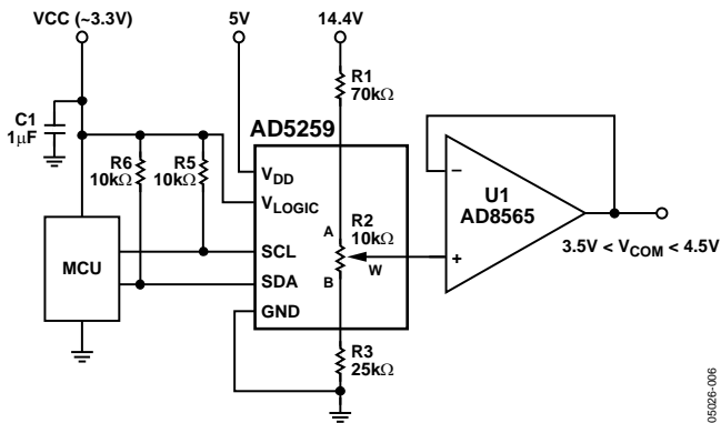
Figure 46. V_{COM} Adjustment Application
