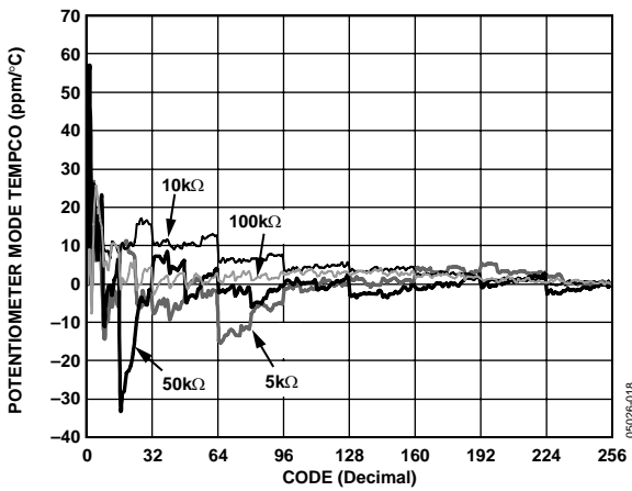
Figure 19. Potentiometer Mode Tempco ( \Delta V_W \times 10^5 )/( V_W \times \Delta T ) vs. Code
