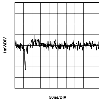
TPC 23. DAC-to-DAC Crosstalk
