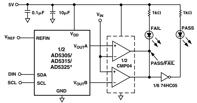
Figure 14. Window Detection
