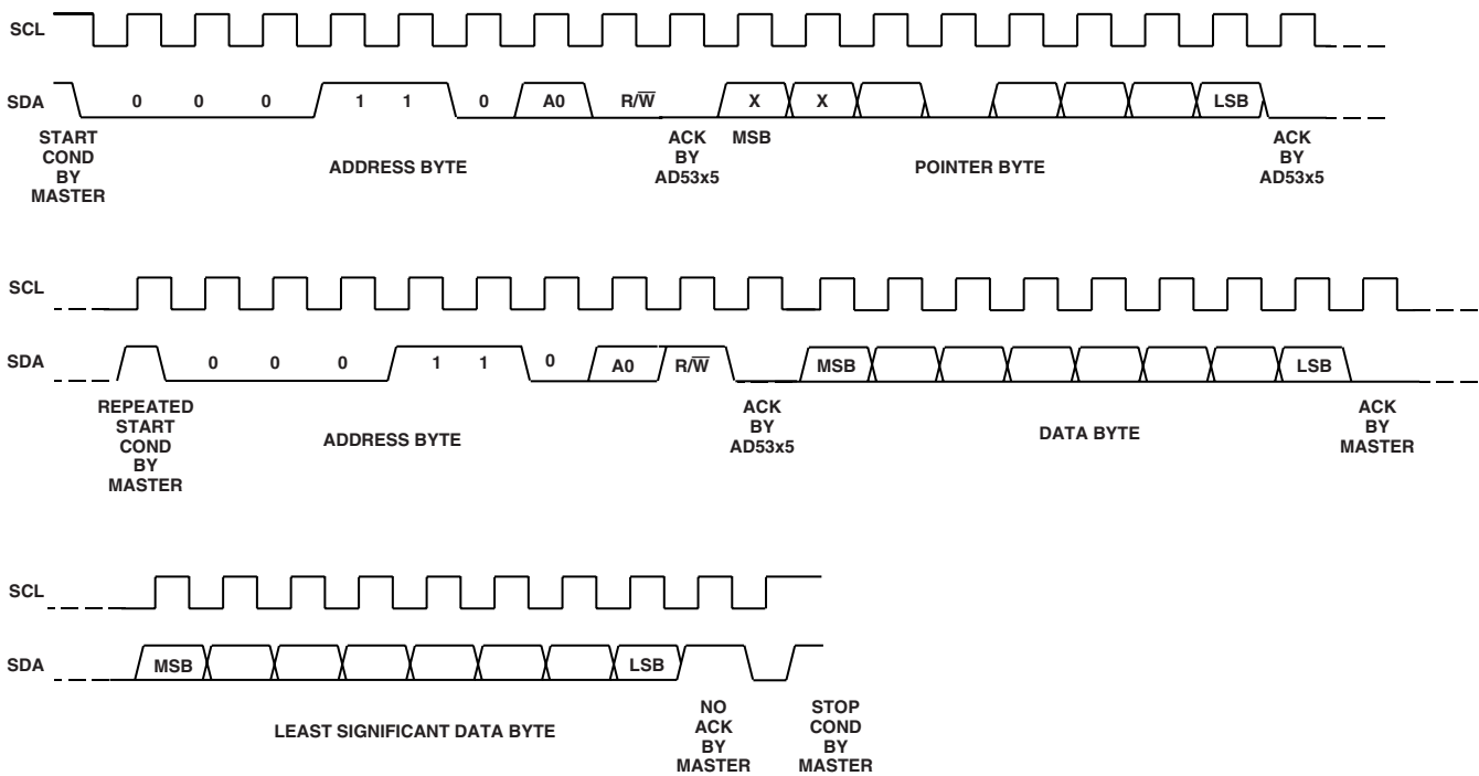
Figure 9. Readback Sequence
